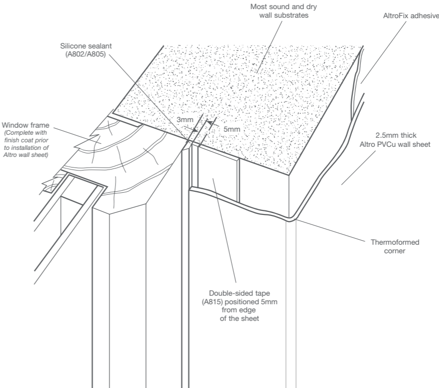
Altro Whiterock hygienic PVCu wall system to shower tray with integral upstand detail
